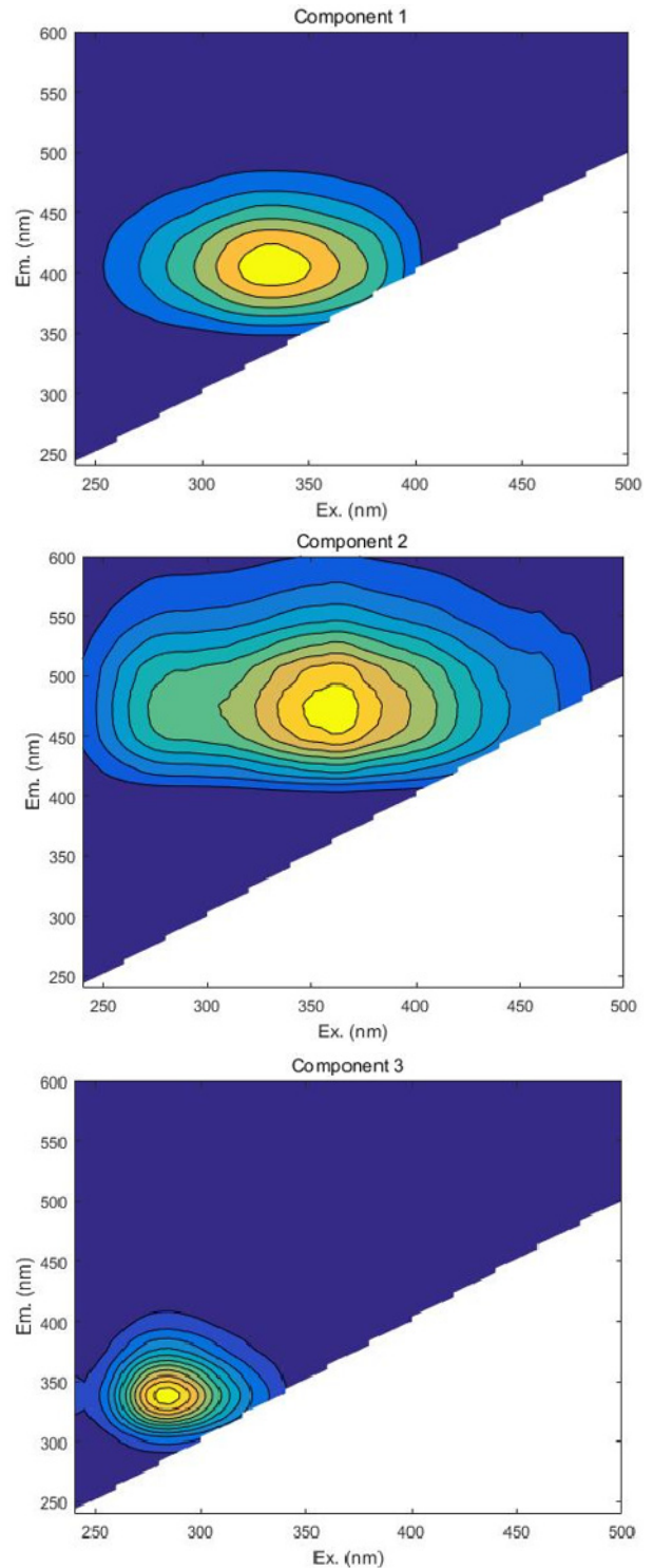
Fig. 4. Excitation-emission matrix spectroscopy (EEMs) contour plots of each component determined by using the parallel factor analysis (PARAFAC) model
